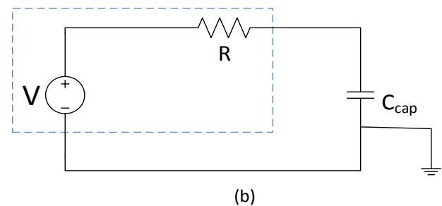
Fig. 2 Schematic diagram of a rectenna: (a) antenna and diode coupled as a rectenna; (b) simplified system equivalent RC circuit.
