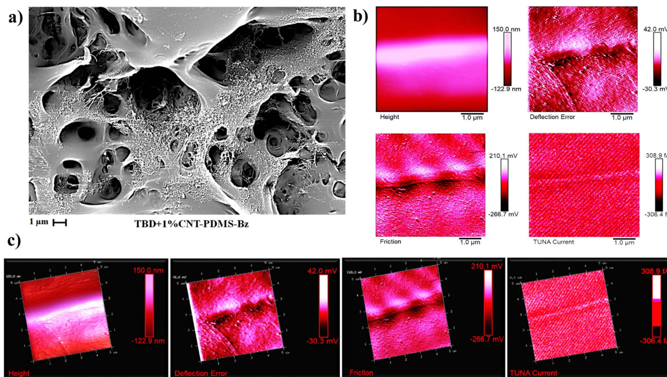
Figure 8. Morphological analysis of the TBD+1%CNT-PDMS-Bz etched fracture surface: (a) FESEM image, (b) the four TUNA-AFM image types, and (c) the corresponding four three-dimensional TUNA-AFM images.
