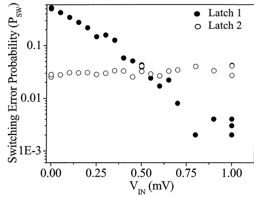
Fig. 9. Variation of the probability of switching errors in a shift register with the magnitude of the input. A bit is written into latch L_1 using the input V_{IN} , and then copied from L_1 to L_2 . This process is repeated for 1000 clock cycles at each value of input. The probability of switching errors in L_1 falls exponentially with V_{IN} while it remains constant for L_2 since L_2 uses L_1 as its input.
