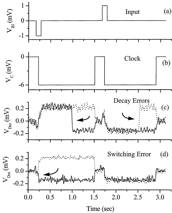
Fig. 7. Errors in the operation of a QCA latch. (a) Input. (b) Clock. (c) Two examples of decay errors (shown by arrows) where information is lost during the clock cycle. (d) Example of a switching error where the latch switches into the wrong state when the clock is applied.
