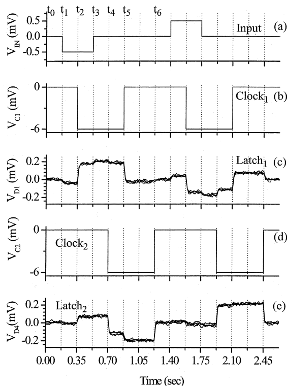
Fig. 5. Operation of a QCA shift register. (a) Input V_{IN} applied to L_1 . (b) Clock V_{C1} to latch L_1 . (c) Output of L_1 measured by the potential on dot D_1 . (d) Phase-shifted clock V_{C2} applied to latch L_2 . (e) Output of L_2 measured by the potential on dot D_4 .
