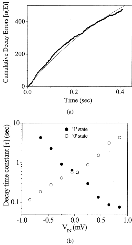
Fig. 8. (a) Cumulative decay errors with respect to time, when the experiment in Fig. 7(c) was repeated for 900 clock cycles. By fitting this data to an exponential saturation curve (dashed line), the bit retention time constant for the latch is found to be 0.52 s. (b) Retention time constant in the bistable region of the phase plot, as a function of the input bias setting.
