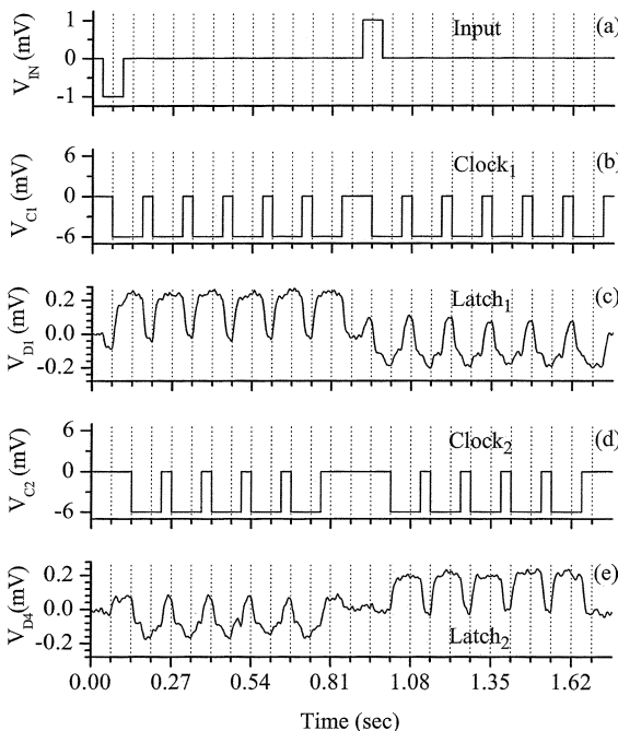
Fig. 6. Simulation of a multistage shift register using a two-stage shift register. A bit is written into latch L_1 by V_{IN} and then by using one latch as input to the other, the bit is copied back and forth to simulate multiple stages. (a) Input applied to L_1 . (b) Clock applied to L_1 . (c) Output of L_1 measured by the potential on dot D_1 . (d) Phase-shifted clock V_{C2} applied to latch L_2 . (e) Output of L_2 measured by the potential on dot D_4 .
