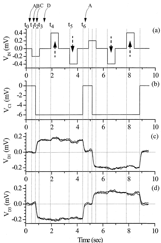
Fig. 4. Operation of a QCA latch. (a) Input applied to D_1 and D_3 ( V_{IN} to D_1 and -V_{IN} to D_3 ). (b) Clock signal V_{C1} applied to the middle dot D_2 . (c) Measured dot potential on D_1 . (d) Measured dot potential on D_3 . Once the latch is in the locked state, disruptive signals (shown by the dotted arrows) twice as large as the original input signal do not affect the state of the latch. Three successive scans are shown in the figure to show the repeatable response.
