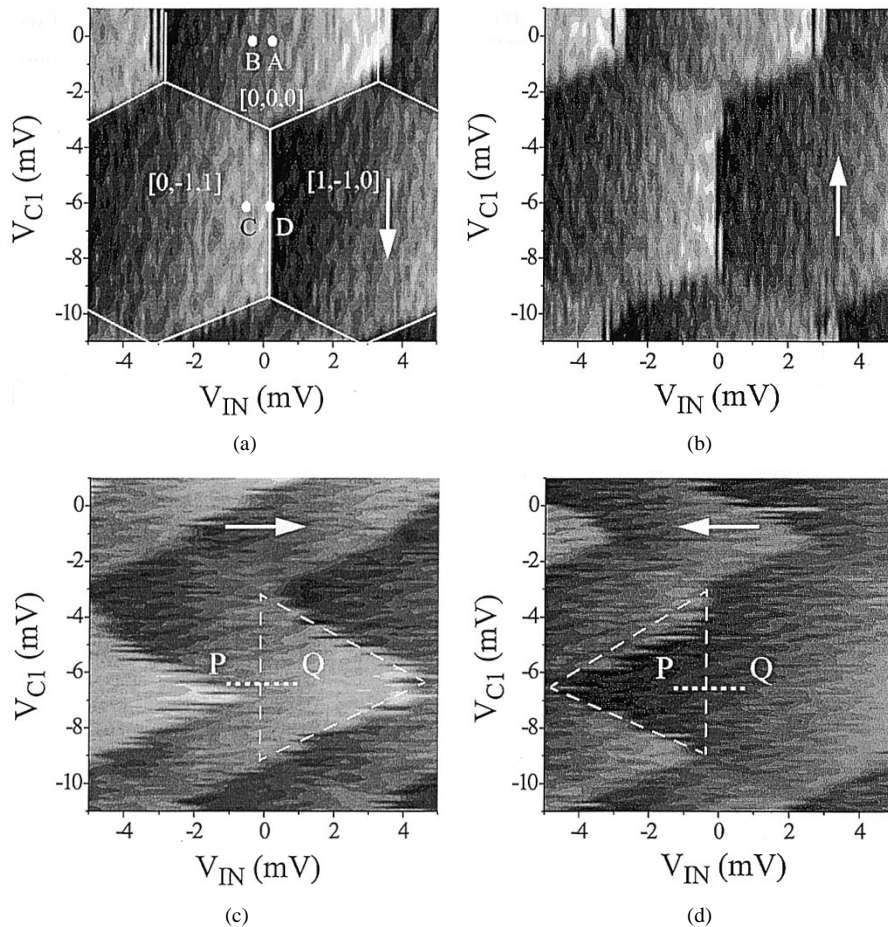
Fig. 3. Phase plot for dot D_1 of latch L_1 for four different scan directions: (a) clock negative, (b) clock positive, (c) input positive, and (d) input negative. Solid white lines represent the boundaries of charge states where electron tunneling occurs. Numbers in brackets (for example [0, -1, 1] ) denote the number of extra electrons in the top, middle, and bottom dots respectively and represent the charge configuration of the latch in that region. Dotted line shows the extent of the bistable region.
