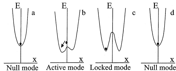
Fig. 1. Simplified diagram of the Keyes-Landauer clocking scheme. Depicts the three main stages involved in varying the potential well from a monostable to a bistable state by modulating a barrier.
