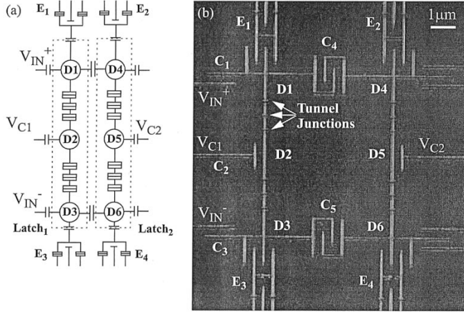
Fig. 2. (a) Schematic diagram of a QCA shift register. (b) Scanning electron micrograph of the shift register.
